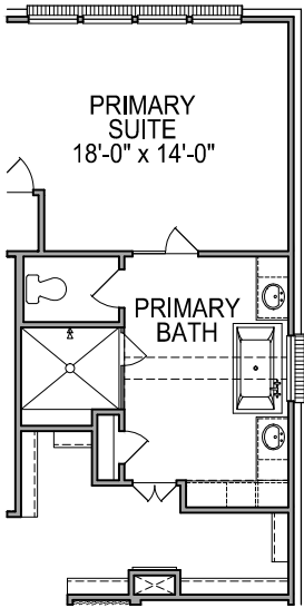
FIRST FLOOR PLAN OPT. #0075 FREE STANDING TUB
