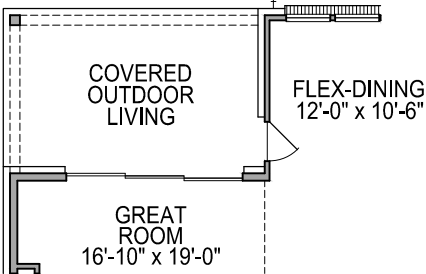
FIRST FLOOR PLAN OPT. #0790 SLIDERS @ GREAT ROOM
