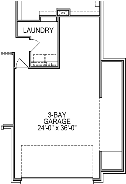
FIRST FLOOR PLAN OPT. #0613 5' GARAGE EXT.
