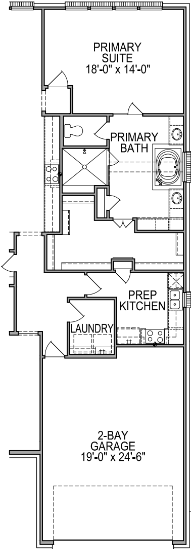
FIRST FLOOR PLAN OPT. #0485 PREP. KITCHEN FROM GARAGE
