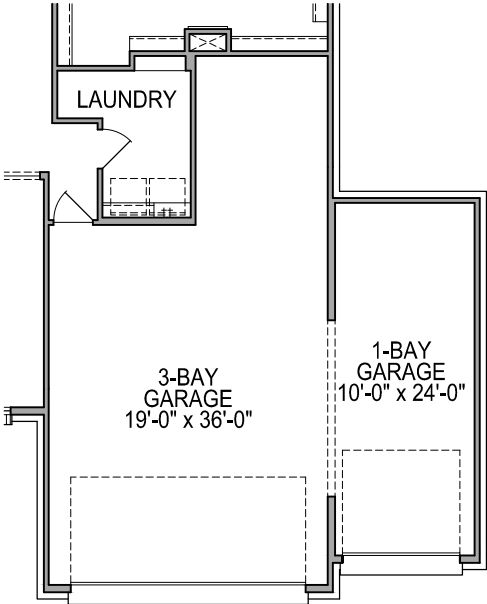
FIRST FLOOR PLAN OPT. #0593 1 BAY GARAGE
