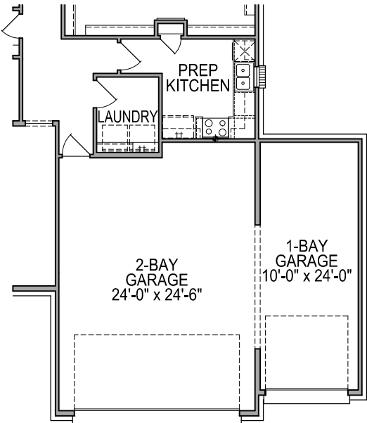
FIRST FLOOR PLAN OPT. #0593 1 BAY GARAGE w/ #0485 PREP. KITCHEN FROM GARAGE
