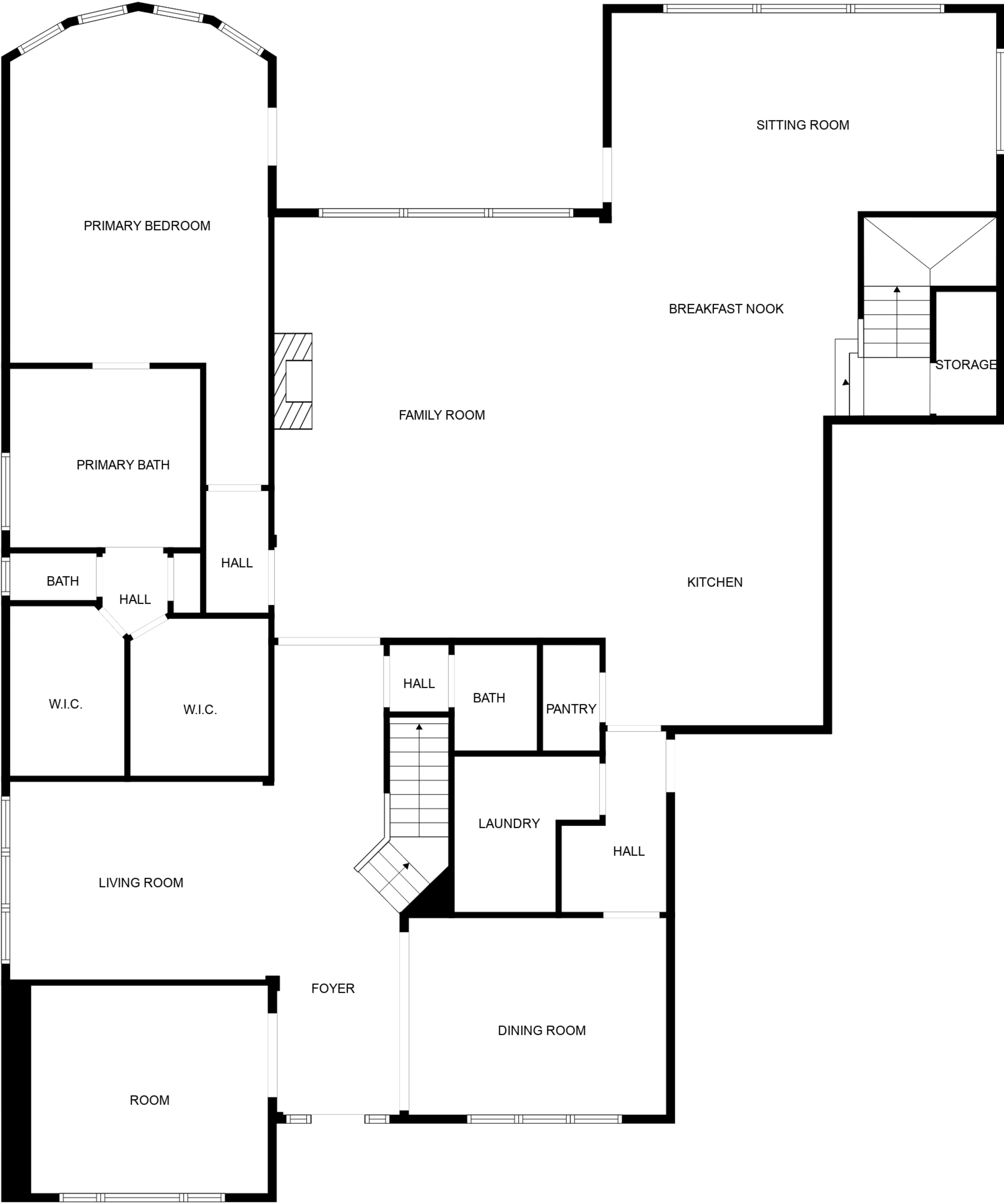
FLOOR 1
