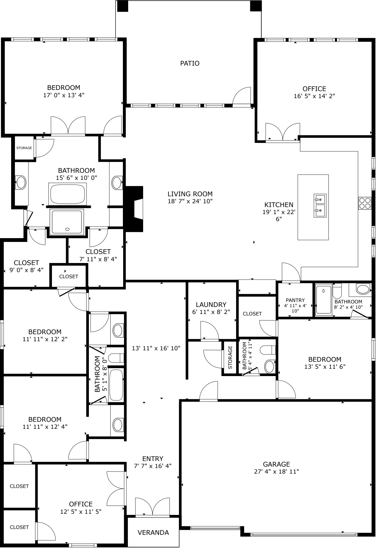
FLOOR PLAN
