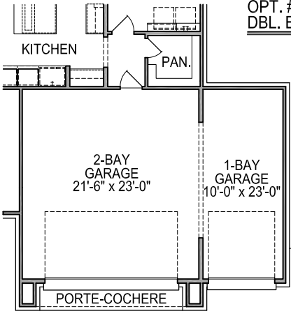
FIRST FLOOR PLAN OPT. #0593 1 BAY GARAGE
