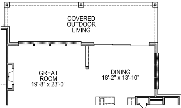
FIRST FLOOR PLAN OPT. #0798 EXT. COVERED OUTDOOR LIVING w/ SLIDERS @ DINING
