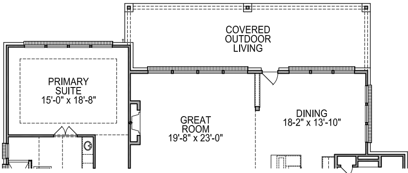
FIRST FLOOR PLAN OPT. #0367 EXTENDED COVERED OUTDOOR LIVING
