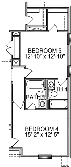
SECOND FLOOR PLAN OPT. #0567 BATH 5
