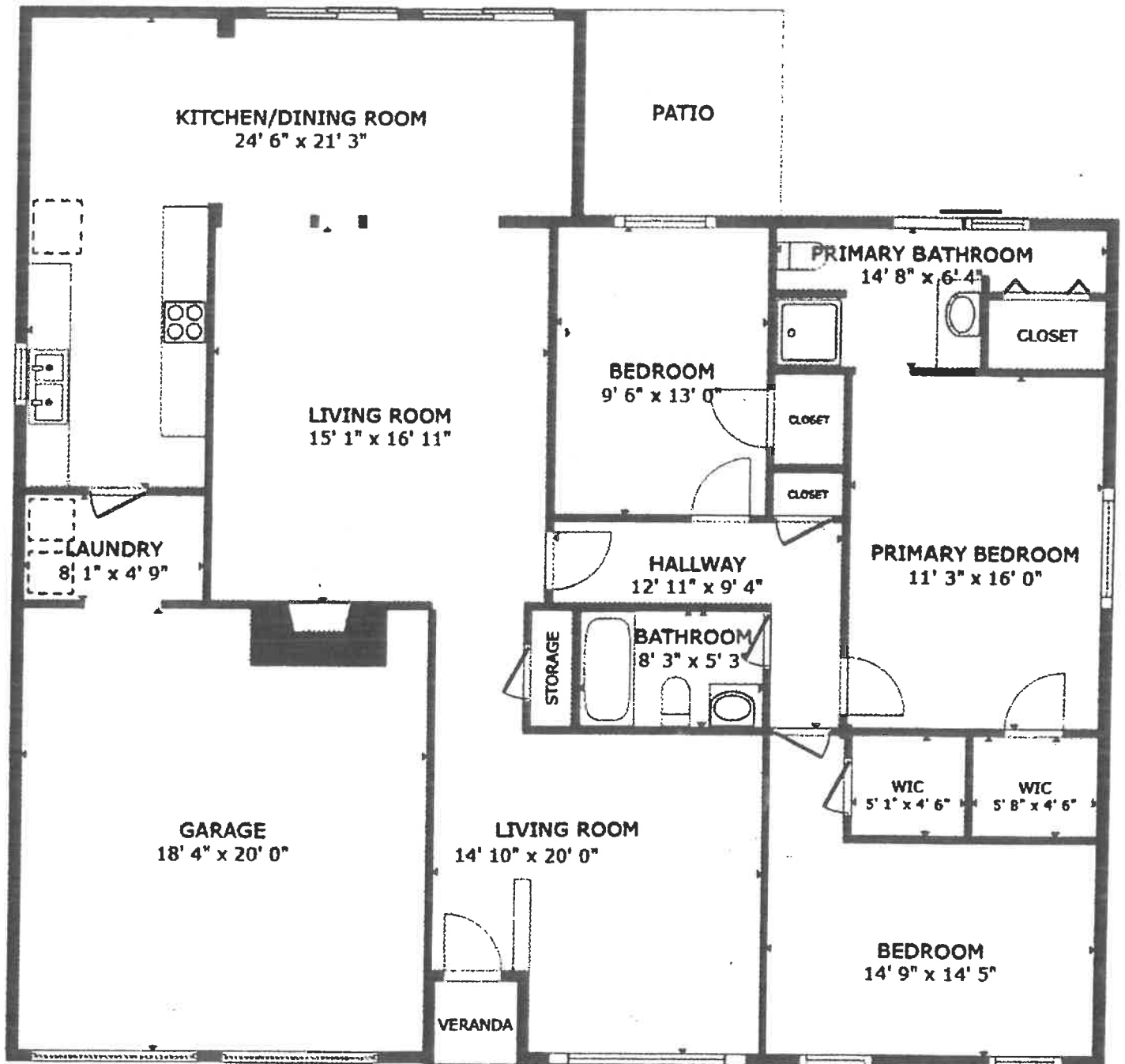
FLOOR PLAN
