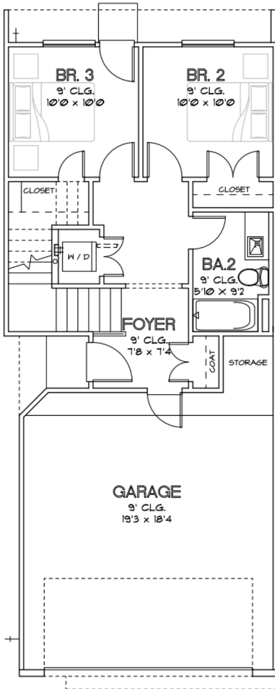
FIRST FLOOR
