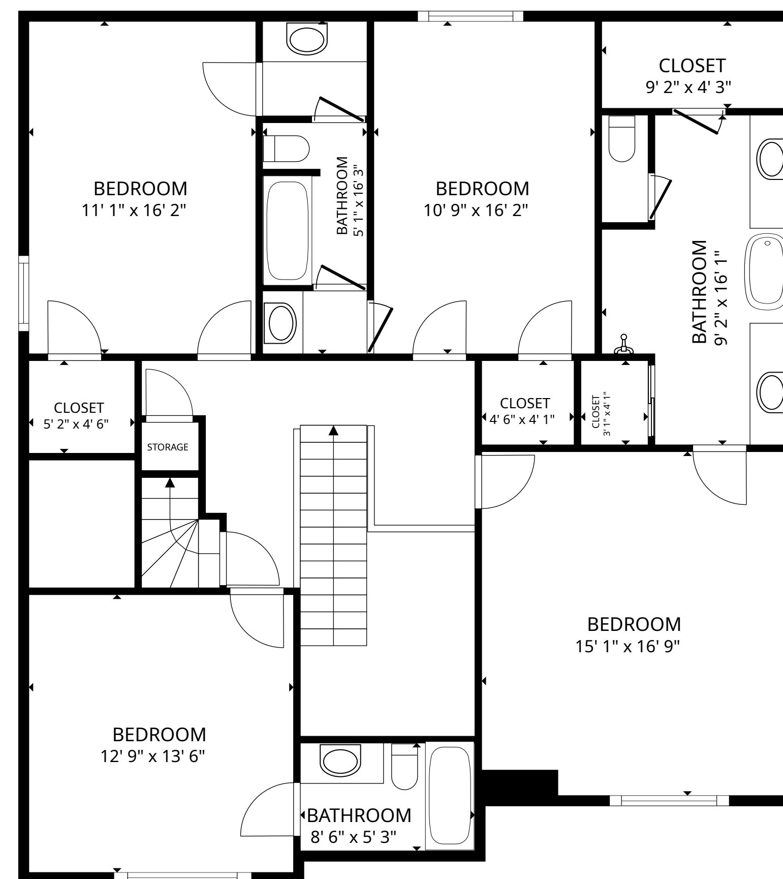
FLOOR 2
