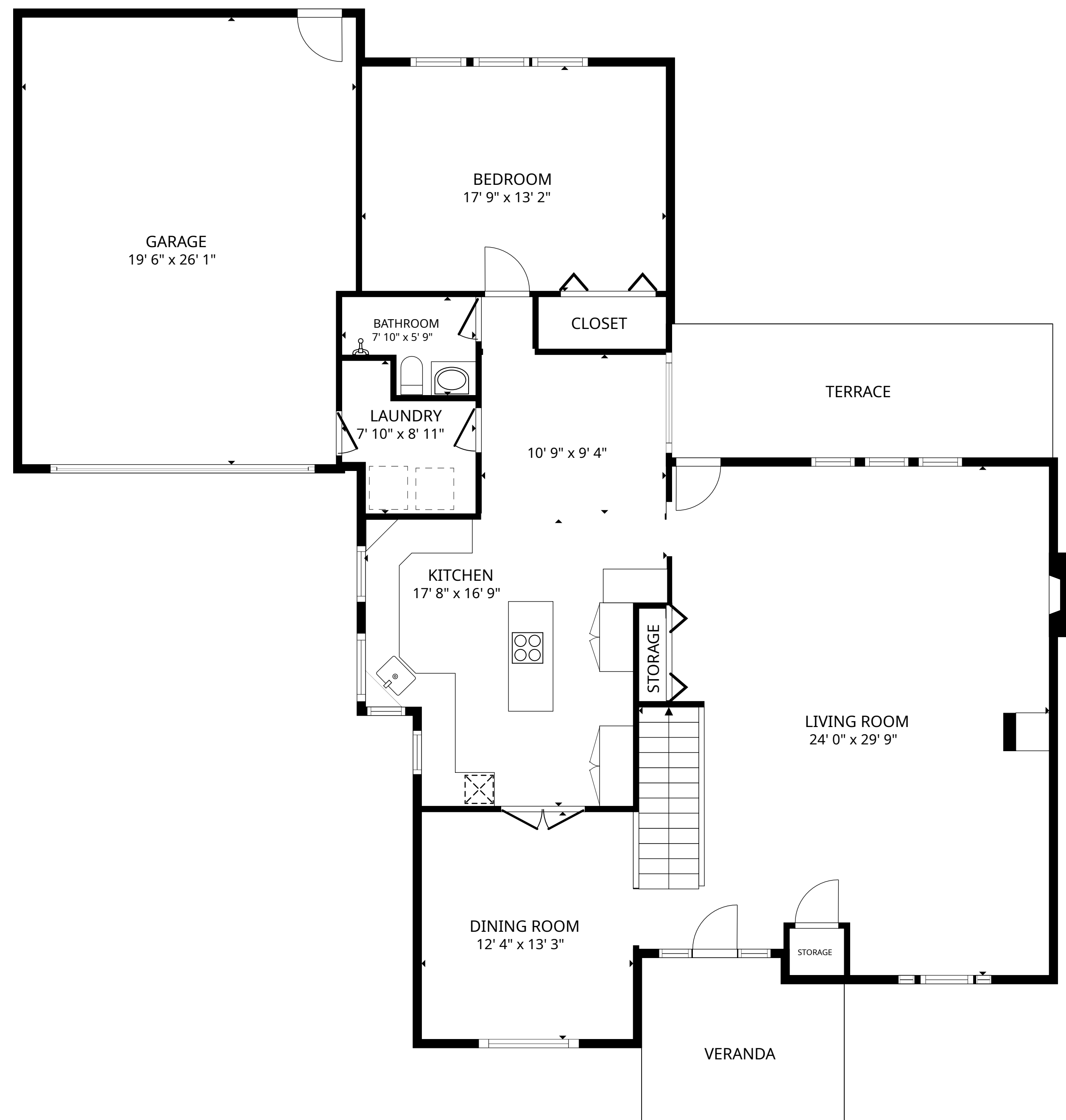
FLOOR 1
