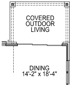
FIRST FLOOR PLAN OPT. #0793 SLIDERS @ DINING
