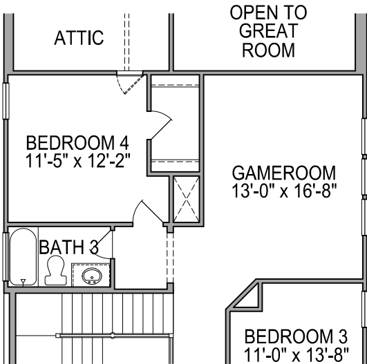
SECOND FLOOR PLAN OPT. #0400 BED 4/BATH 3 FROM ATTIC
