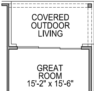
FIRST FLOOR PLAN OPT. #0795 COVERED OUTDOOR LIVING w/ GREAT ROOM SLIDERS
