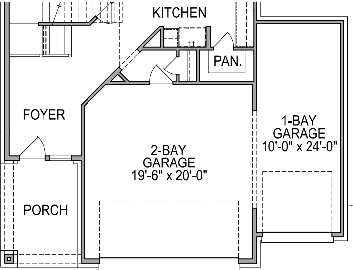
FIRST FLOOR PLAN OPT. #0593 1 BAY GARAGE
