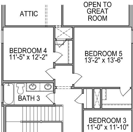
SECOND FLOOR PLAN OPT. #0459 BED 4 & 5/BATH 3 FROM GAMEROOM
