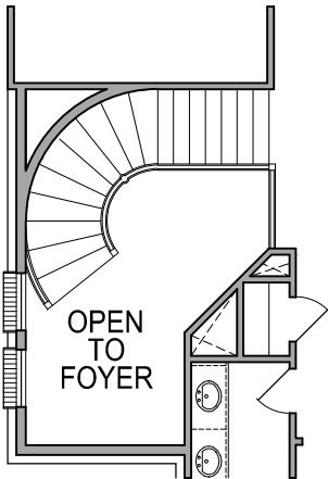
SECOND FLOOR PLAN OPT. #0113 CURVED STAIRS
