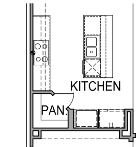
FIRST FLOOR PLAN OPT. #KITUPGSI 36" COOKTOP w/ OVEN/MICRO TOWER CONFIGURATION
