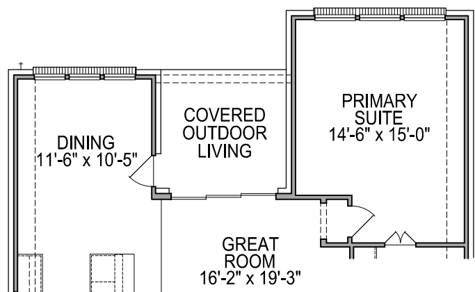
FIRST FLOOR PLAN OPT. #0790 SLIDERS @ GREAT ROOM
