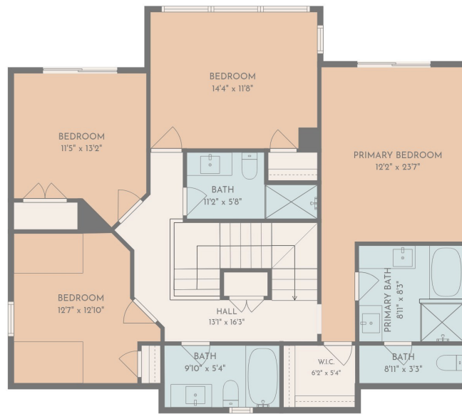
2nd floor
