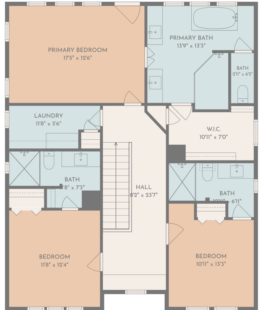
2nd floor
