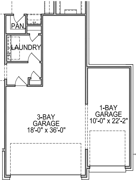
FIRST FLOOR PLAN OPT. #0593 1 BAY GARAGE
