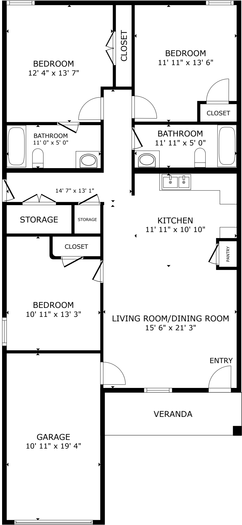
FLOOR PLAN
