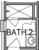
FIRST FLOOR PLAN OPT. #0155 SHOWER AT BATH 2
