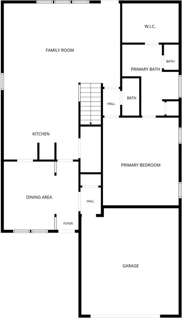
1st floor
