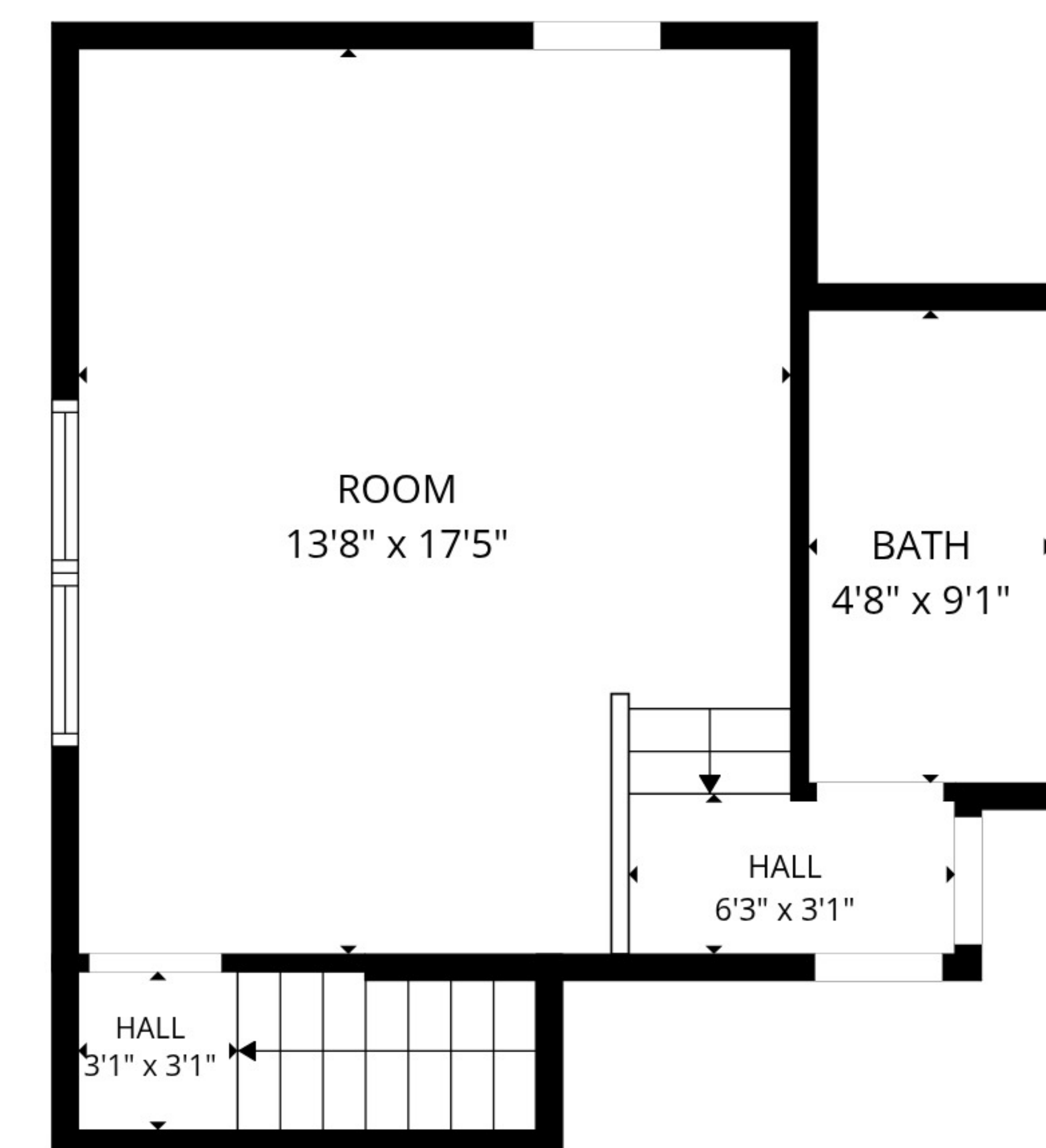
2nd floor
