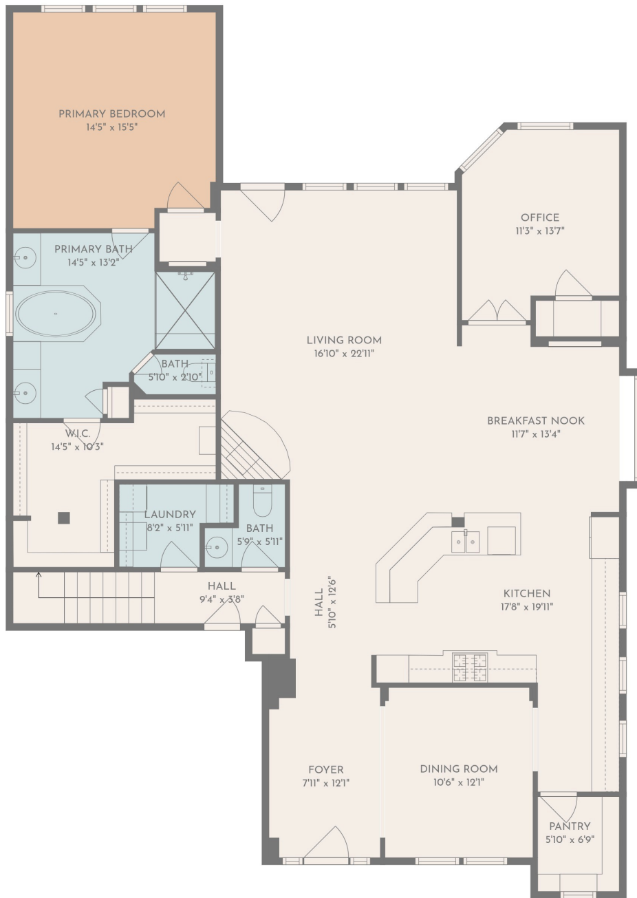
FLOOR 1
