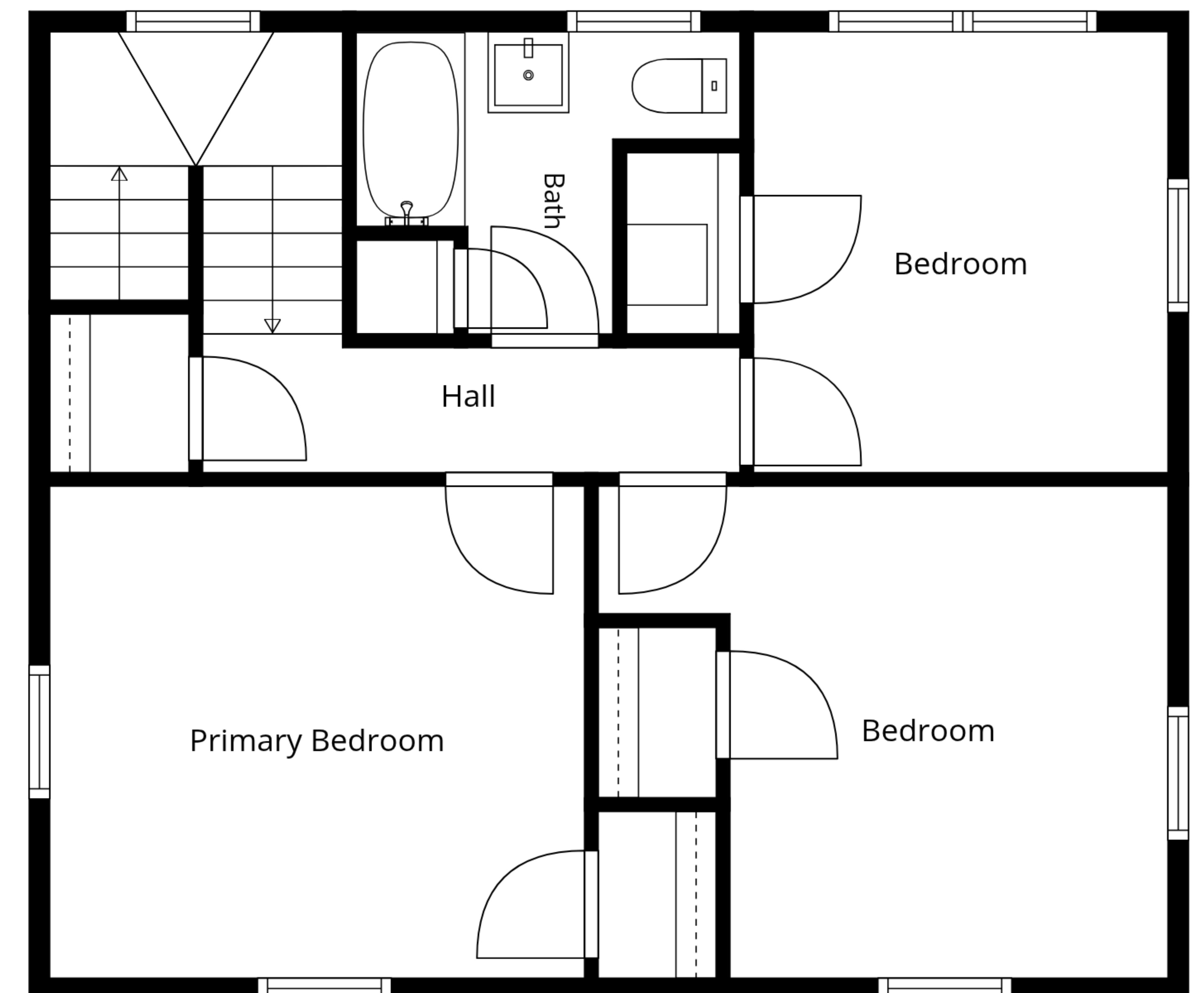
2nd Floor
