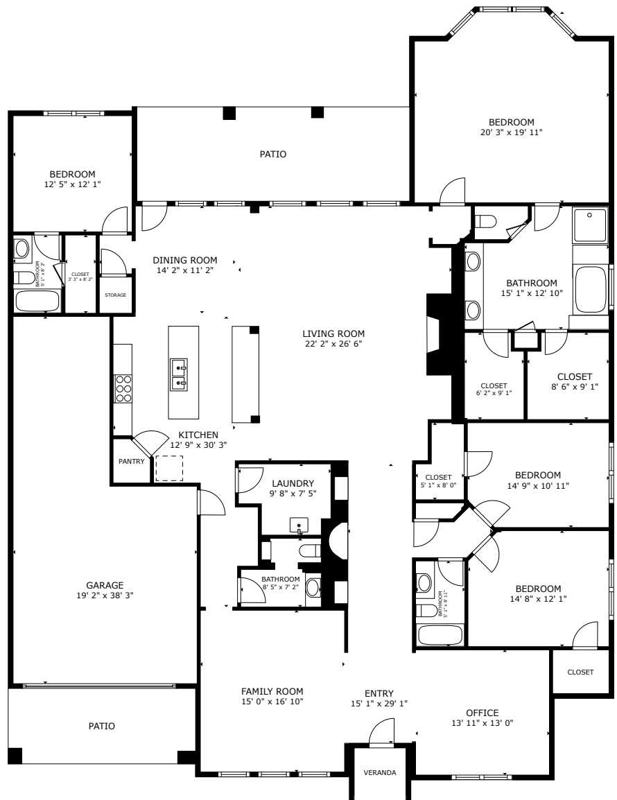
FLOOR PLAN
