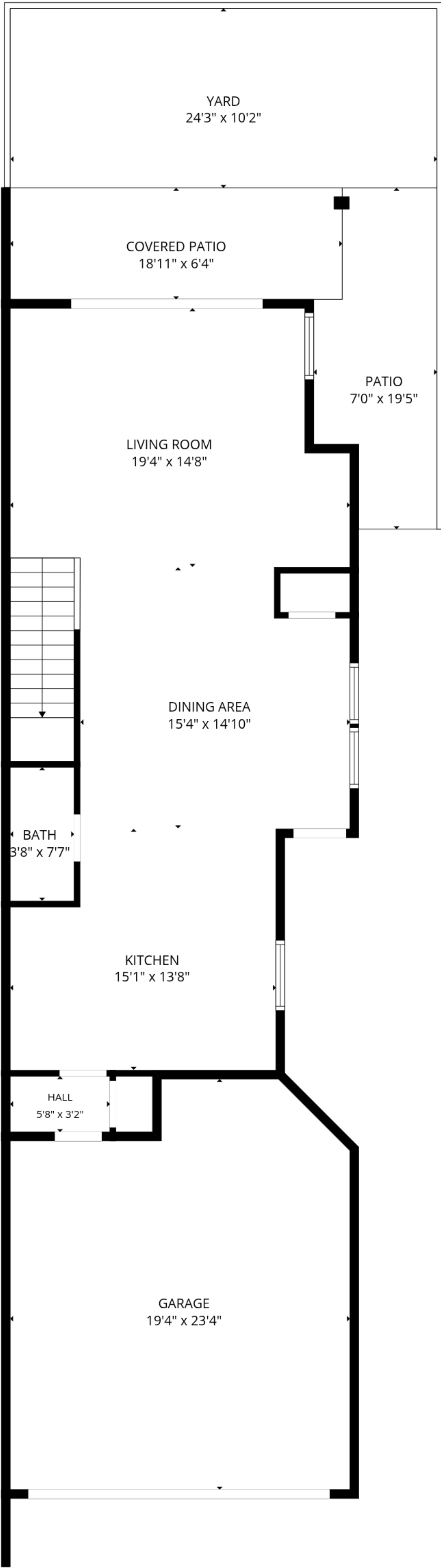
1st floor
