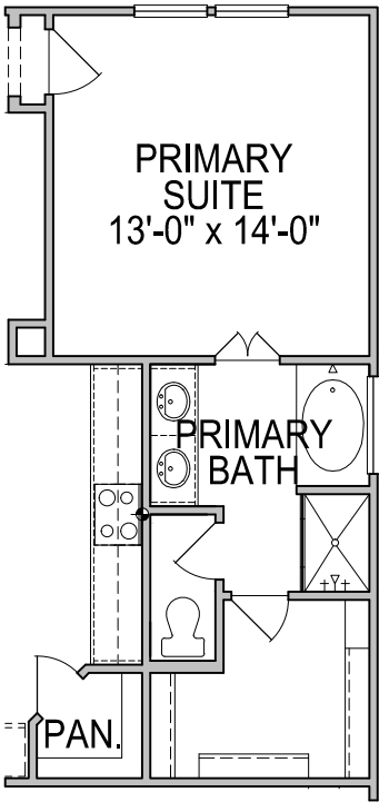
FIRST FLOOR PLAN OPT. #0751 PRIMARY BATH TUB
