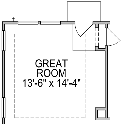
FIRST FLOOR PLAN OPT. #0714 GREAT ROOM COFFER
