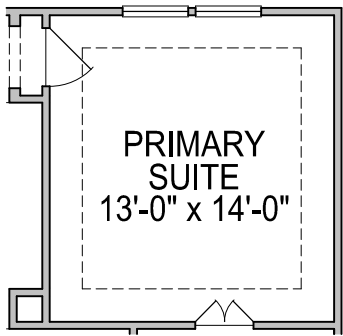
FIRST FLOOR PLAN OPT. #0668 PRIMARY SUITE COFFER
