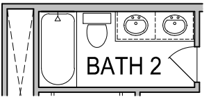
SECOND FLOOR PLAN OPT. #0308 DBL. SINKS @ BATH 2
