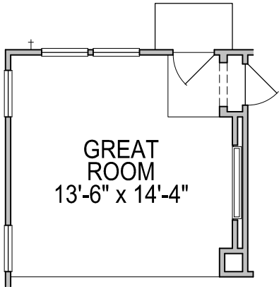
FIRST FLOOR PLAN OPT. #0160 ELECTRIC FIREPLACE
