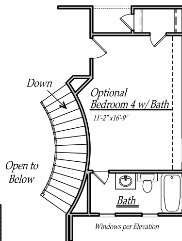
Second Floor Optional Bathroom 4 Additional 98 sq/ft
