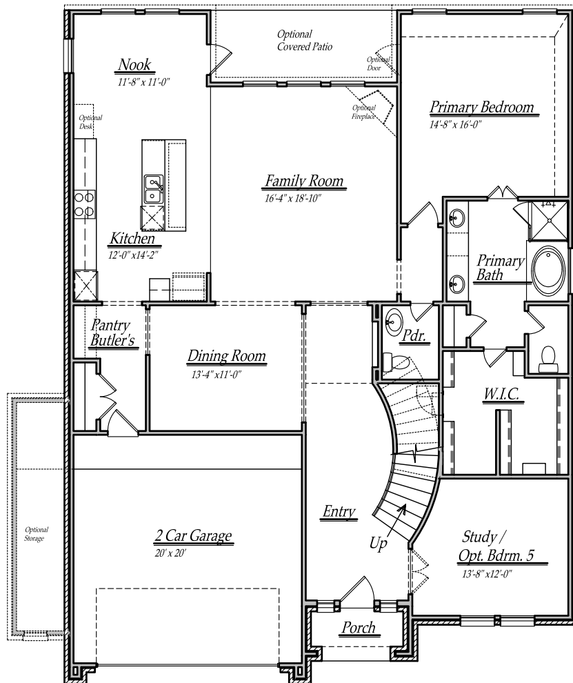
First Floor
