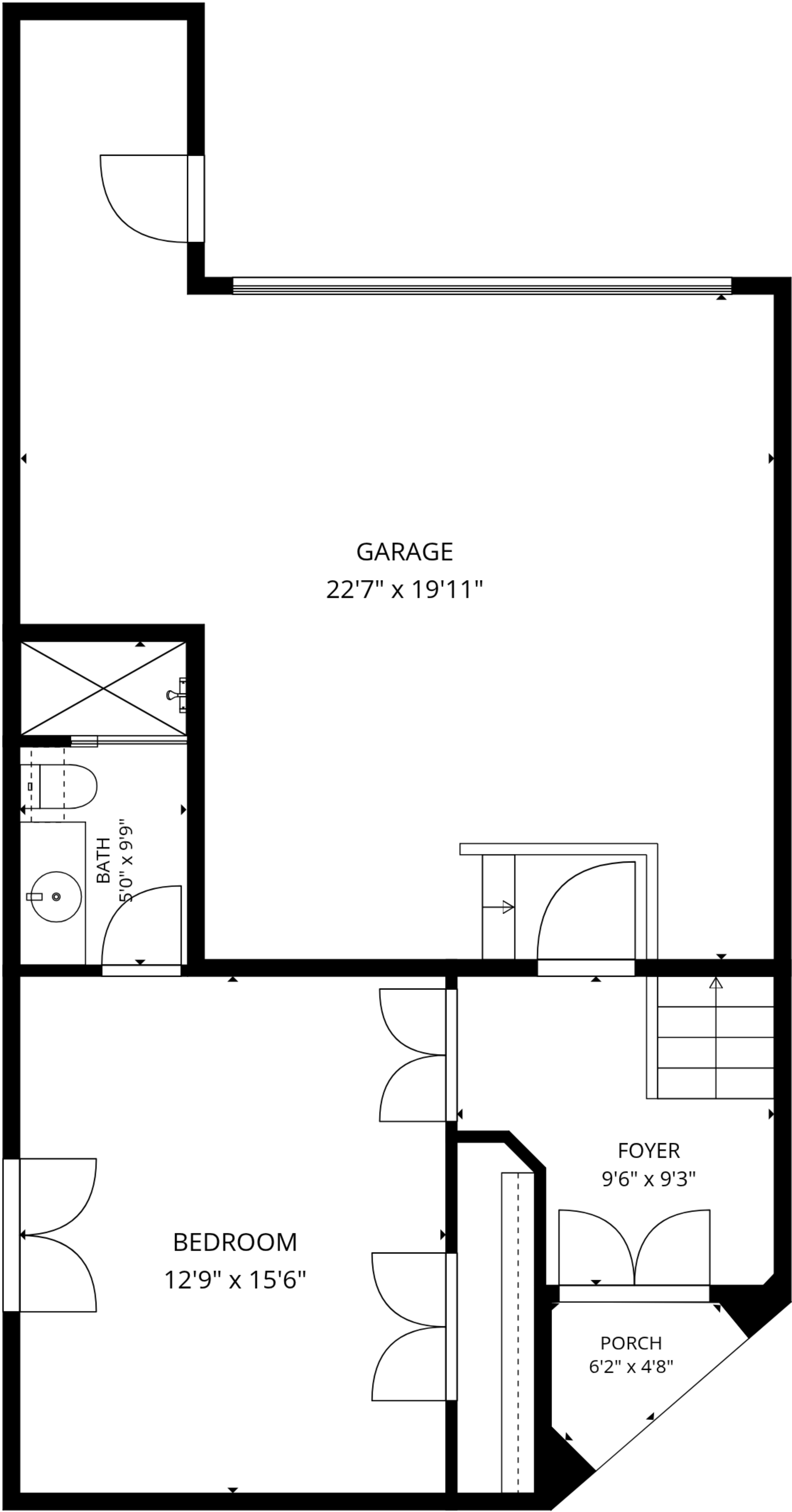
1st floor
