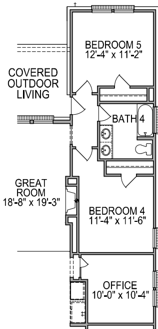
FIRST FLOOR PLAN OPT. #0094 BEDROOM 5 FROM GAMEROOM
