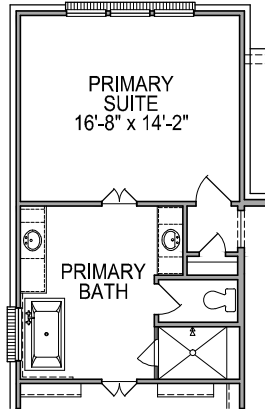
FIRST FLOOR PLAN OPT. #0075 FREE STANDING TUB
