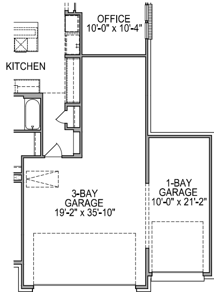
FIRST FLOOR PLAN OPT. #0593 1 BAY GARAGE
