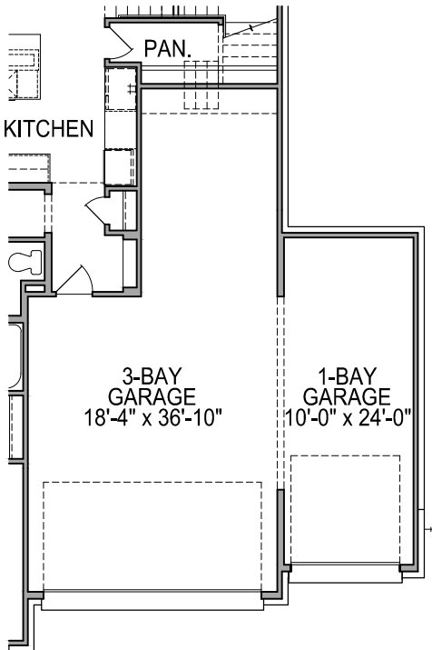
FIRST FLOOR PLAN OPT. #0593 1 BAY GARAGE
