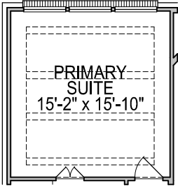
FIRST FLOOR PLAN OPT. BEAMS @ PRIMARY SUITE
