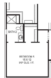
OPTIONAL BEDROOM 5 WITH SHOWER ADDED TO BATH 2 IN LIEU OF STUDY
