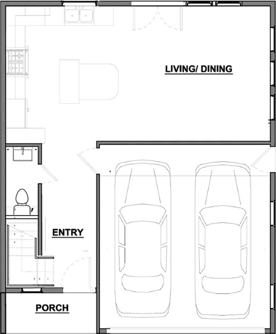
FIRST FLOOR PLAN (A)
