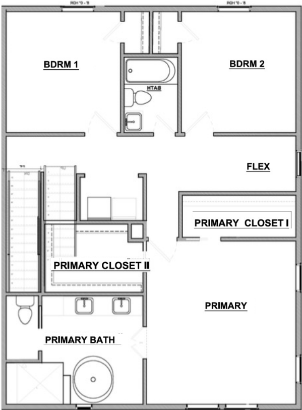
SECOND FLOOR PLAN (B)
