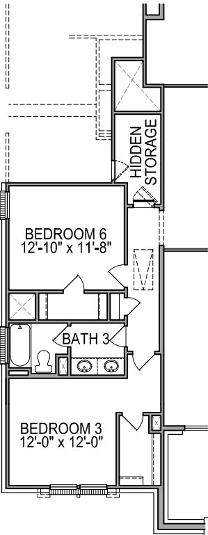
SECOND FLOOR PLAN OPT. #0755 BED 6 FROM MEDIA
