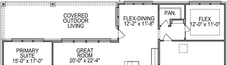
FIRST FLOOR PLAN OPT. #0367 EXT. COVERED OUTDOOR LIVING
