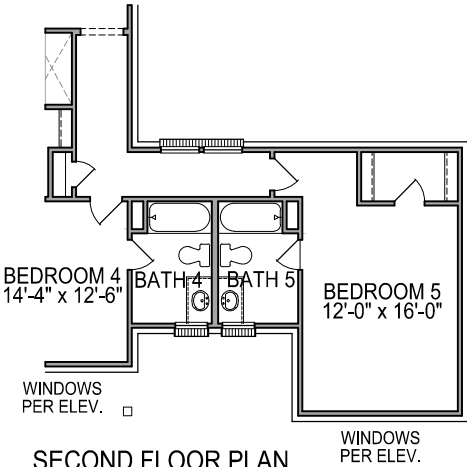
SECOND FLOOR PLAN OPT. #0567 BATH 5 FROM BATH 4
