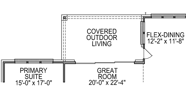
FIRST FLOOR PLAN OPT. #0790 SLIDERS @ GREAT ROOM
