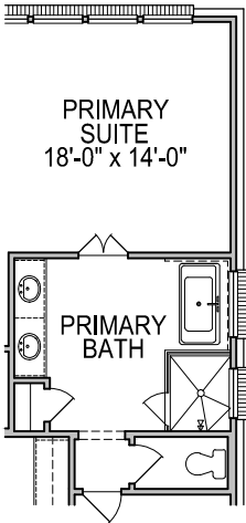
FIRST FLOOR PLAN OPT. #0073 5' FREE STANDING TUB
