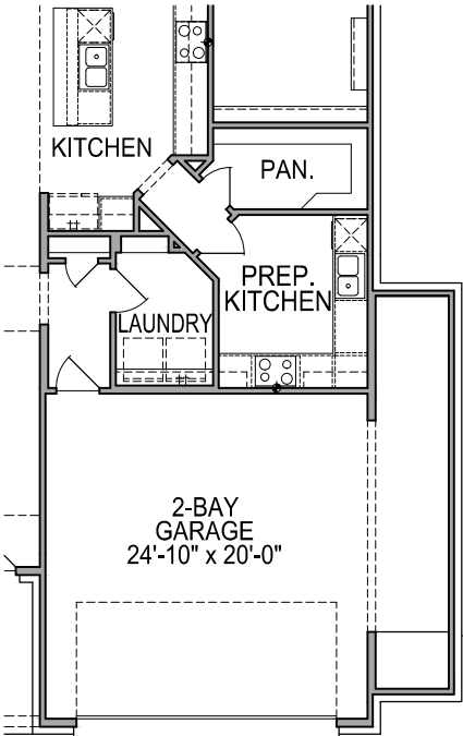
FIRST FLOOR PLAN OPT. #0485 PREP KITCHEN w/ OPT. #0613 5' GARAGE EXT. FROM GARAGE
