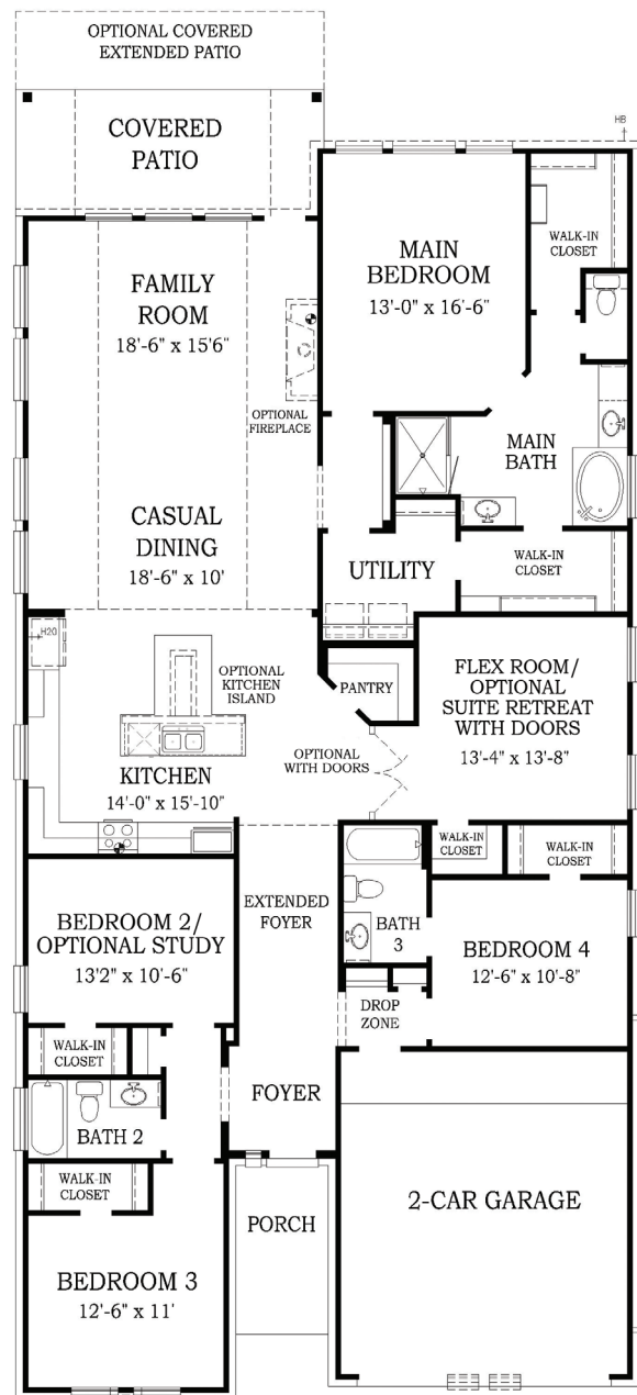
FLOOR PLAN
