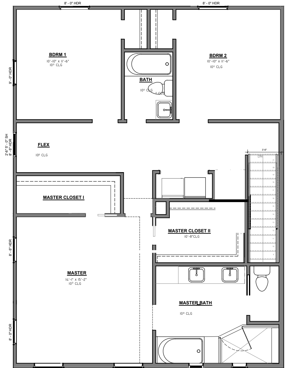
SECOND FLOOR PLAN (B) 1050sf
