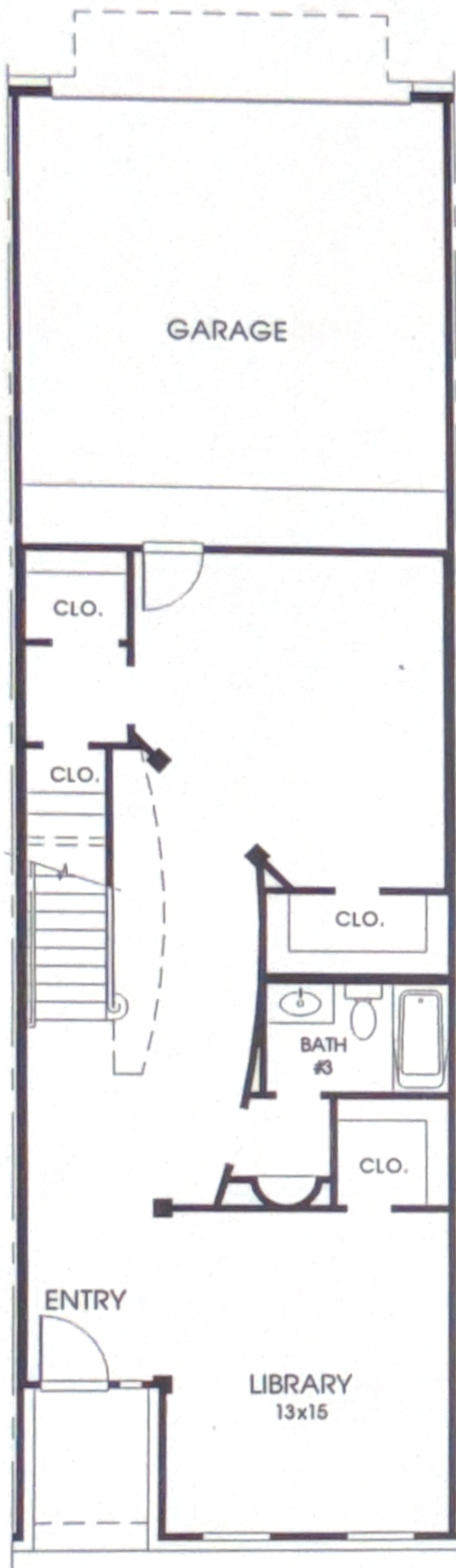
FIRST FLOOR
