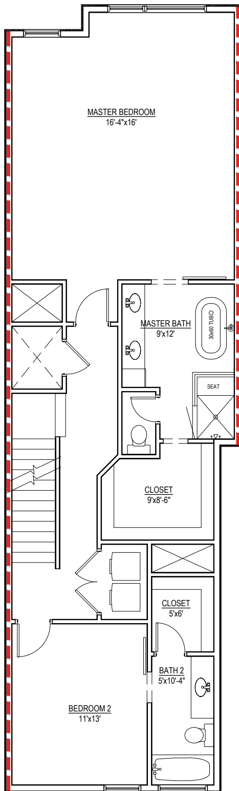
THIRD FLOOR
