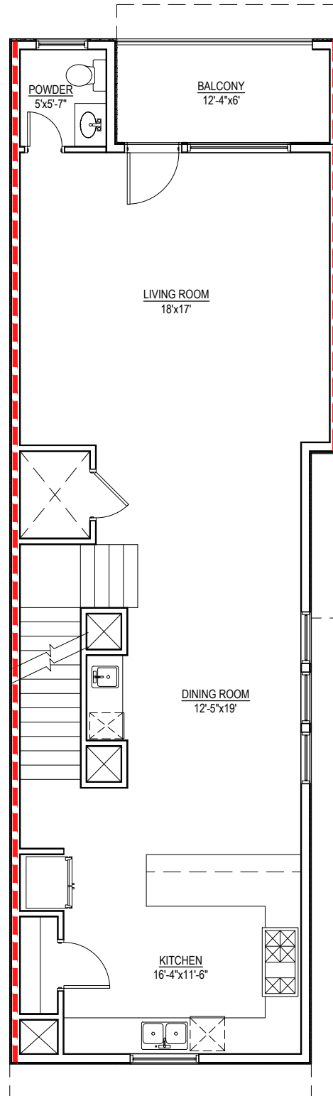
SECOND FLOOR
