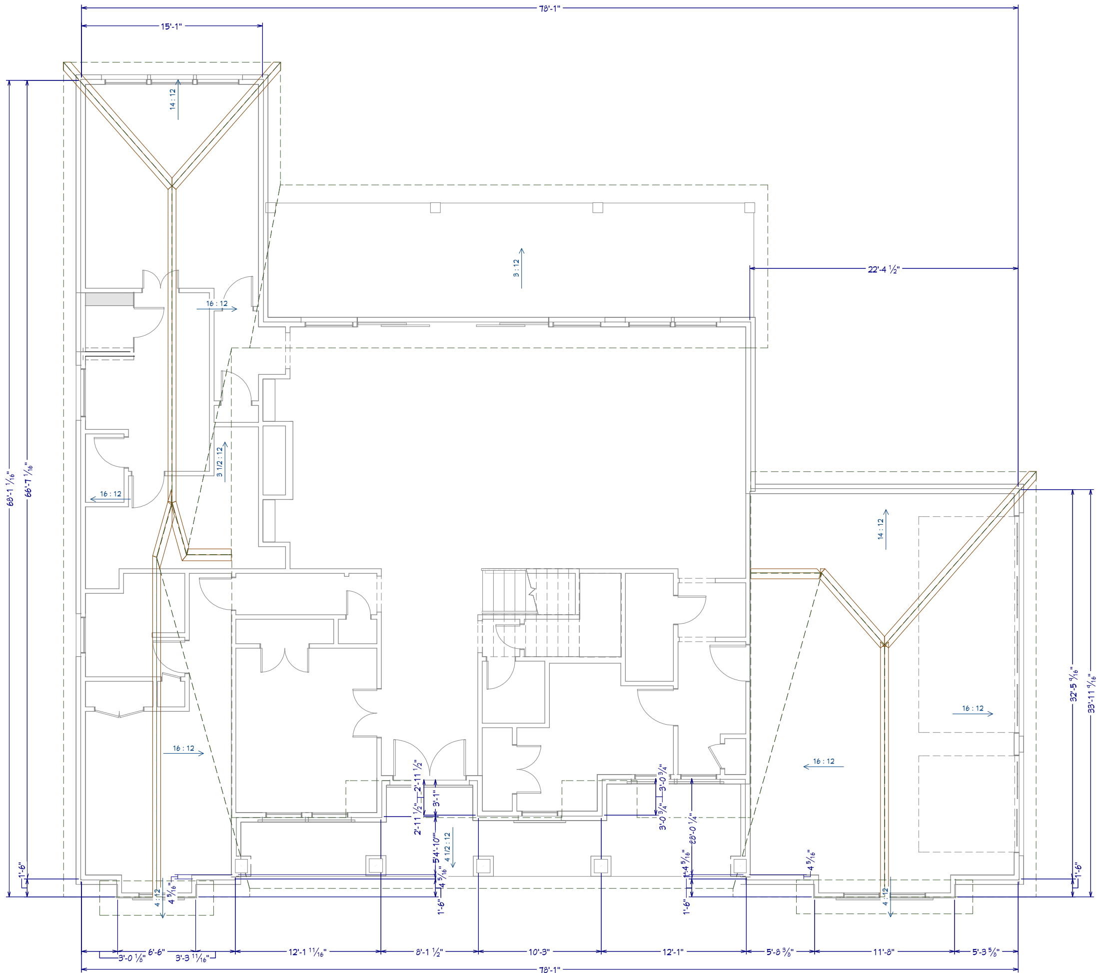
Roof 1st Floor - 1/8 in = 1 ft
