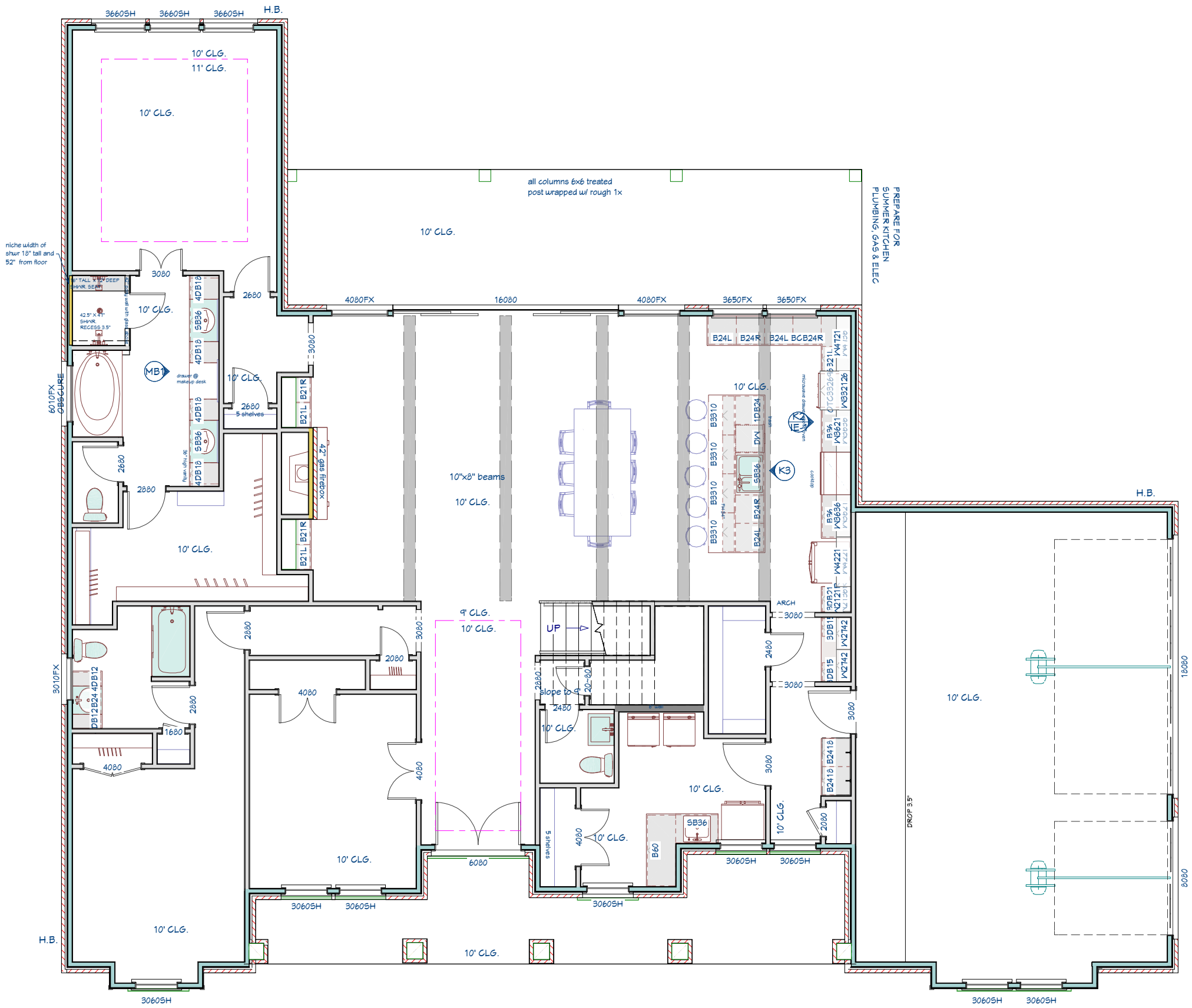
FIRST FLOOR - 1/8 in = 1 ft
