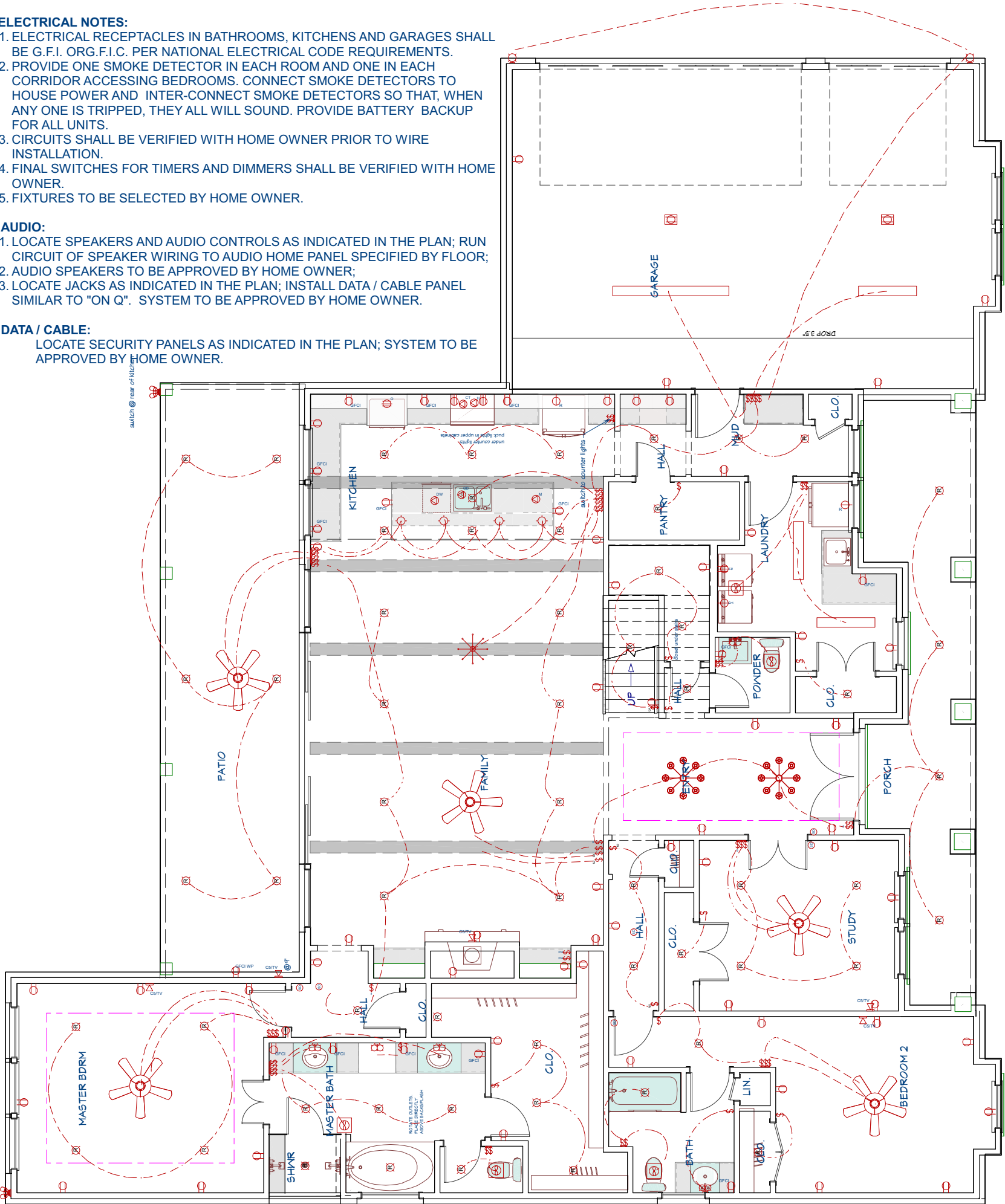
Electrical Plan View
