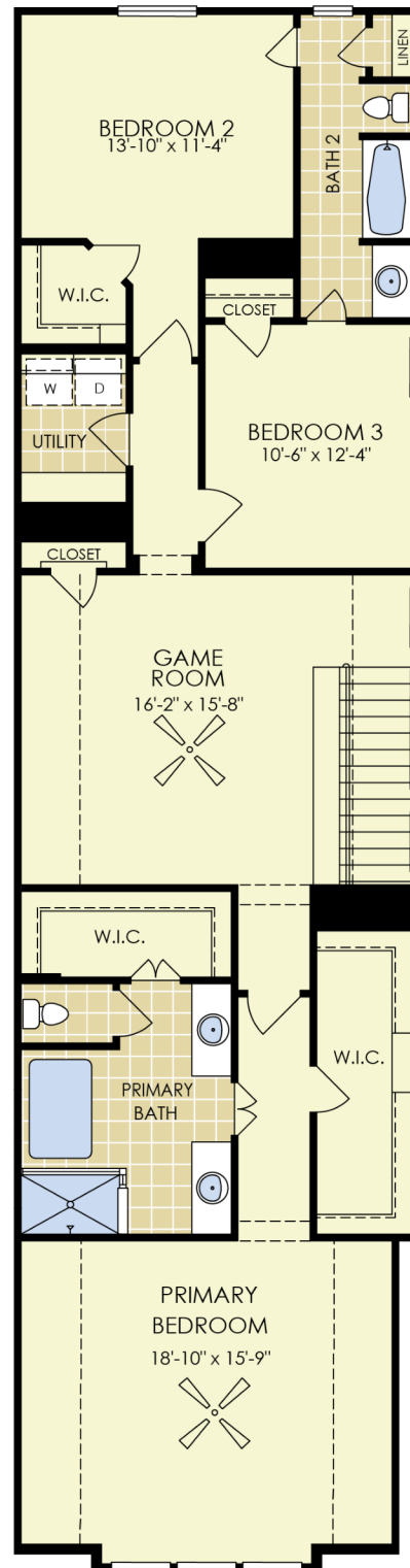
SECOND FLOOR
