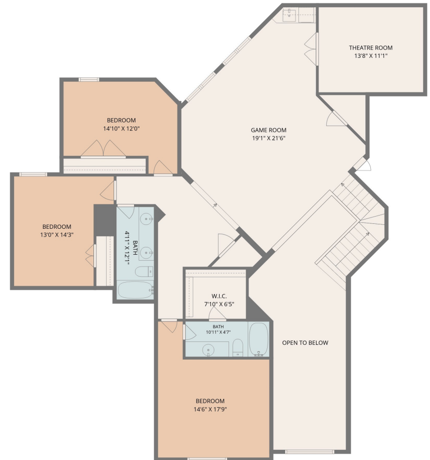
2ND FLOOR
