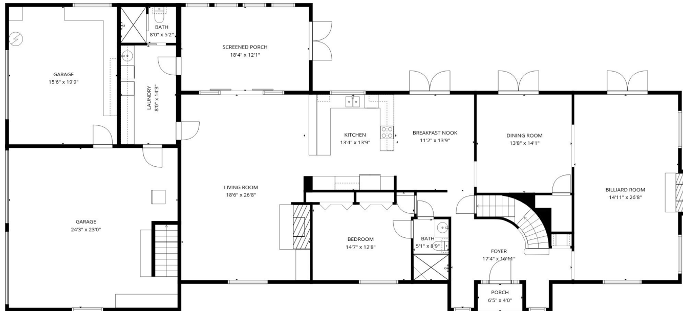
1st floor
