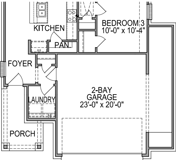
FIRST FLOOR PLAN OPT. #0613 5' GARAGE EXT.
