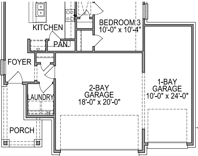
FIRST FLOOR PLAN OPT. #0593 1 BAY GARAGE
