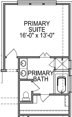
FIRST FLOOR PLAN OPT. #0071 LUXURY PRIMARY BATH
