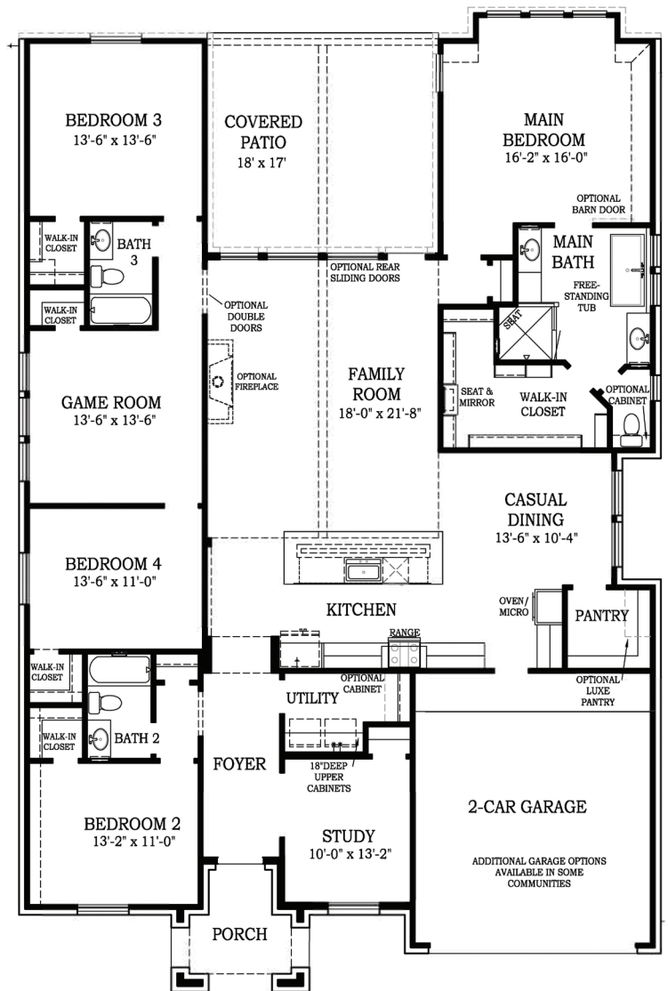
FLOOR PLAN
