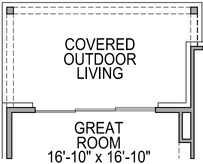
FIRST FLOOR PLAN OPT. #0795 COVERED OUTDOOR LIVING w/ GREAT ROOM SLIDERS
