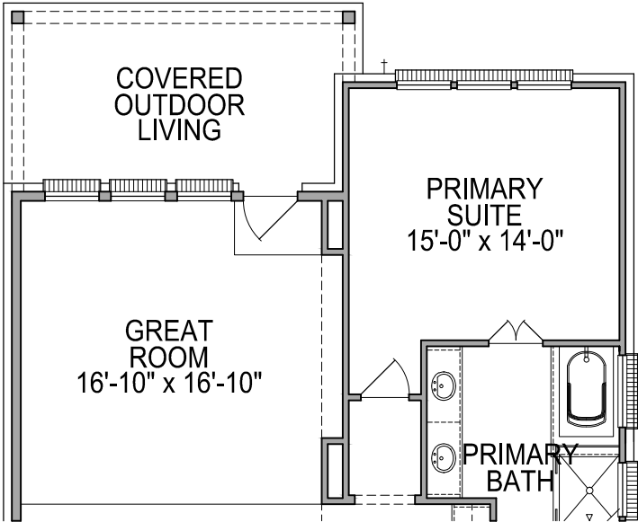
FIRST FLOOR PLAN OPT. #0105 COVERED OUTDOOR LIVING
