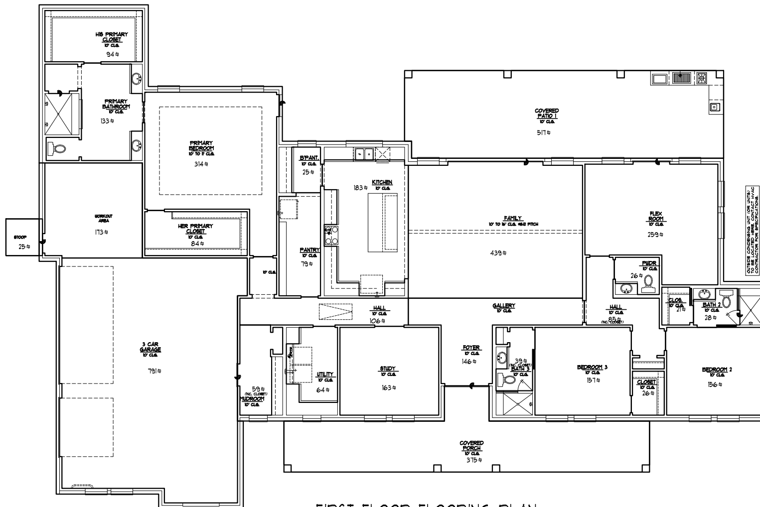
FIRST FLOOR FLOORING PLAN SCALE: 1/4"=1'-0"
