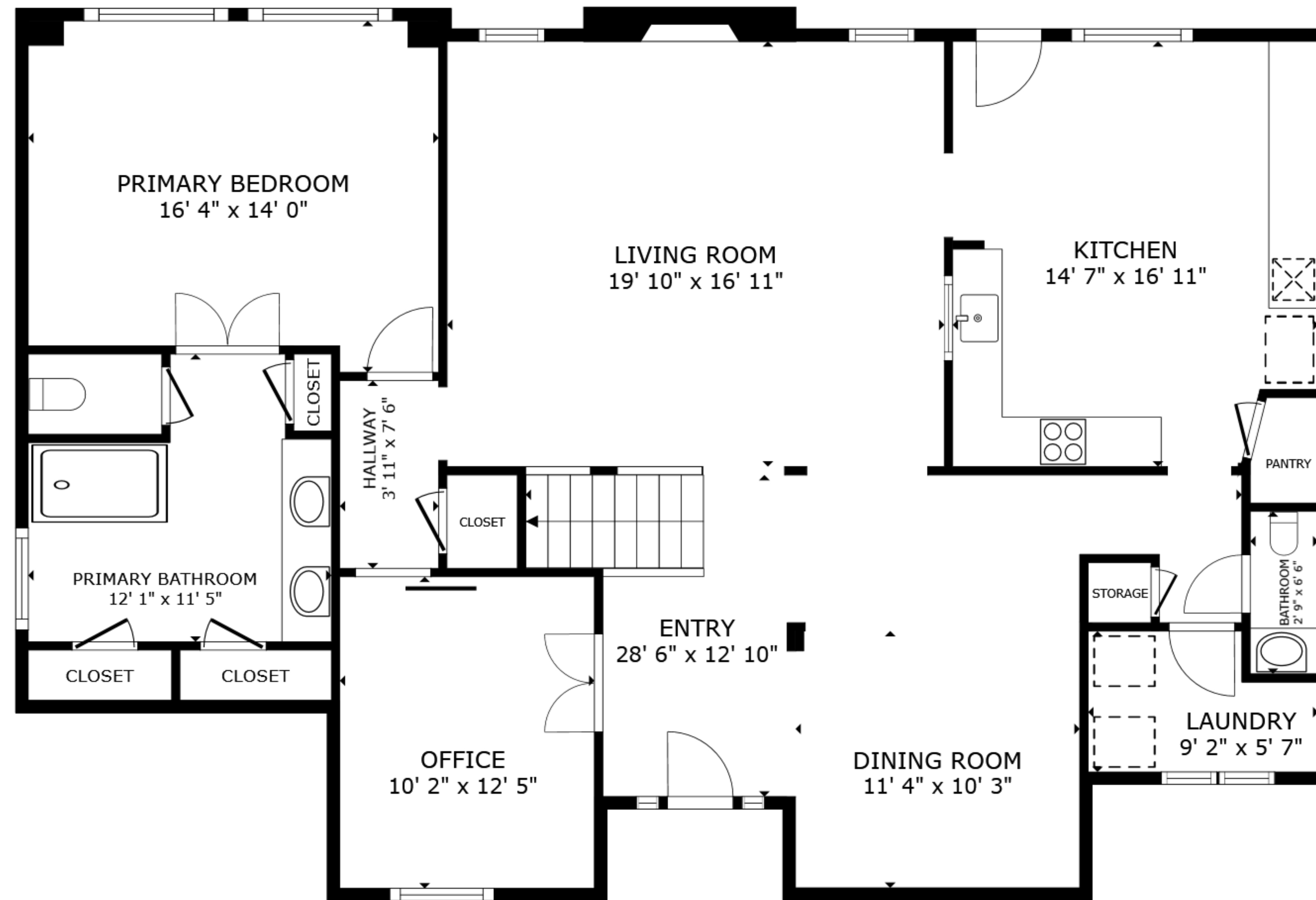
FLOOR 1
