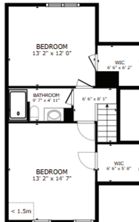
FLOOR 2
