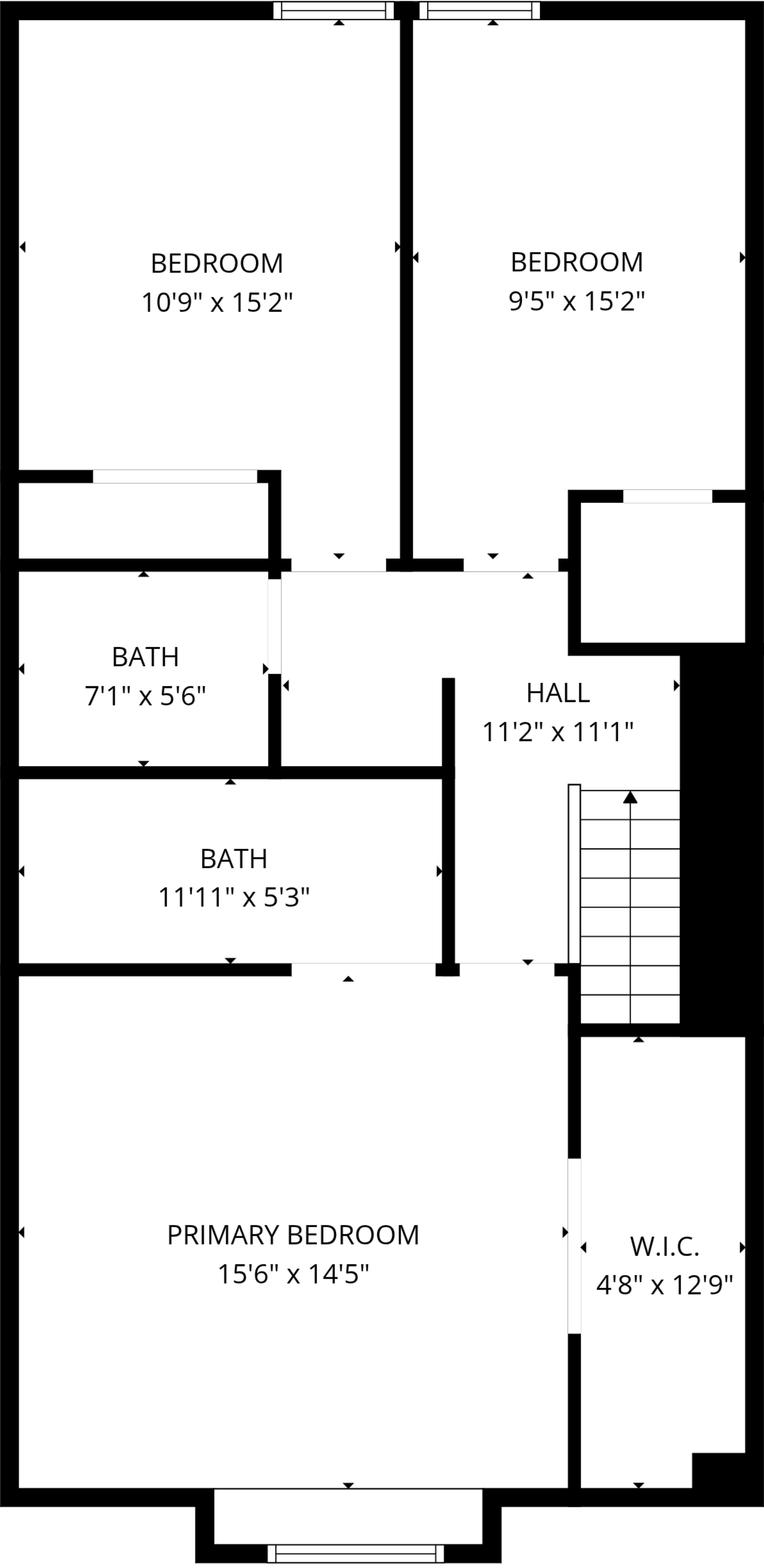
2nd floor
