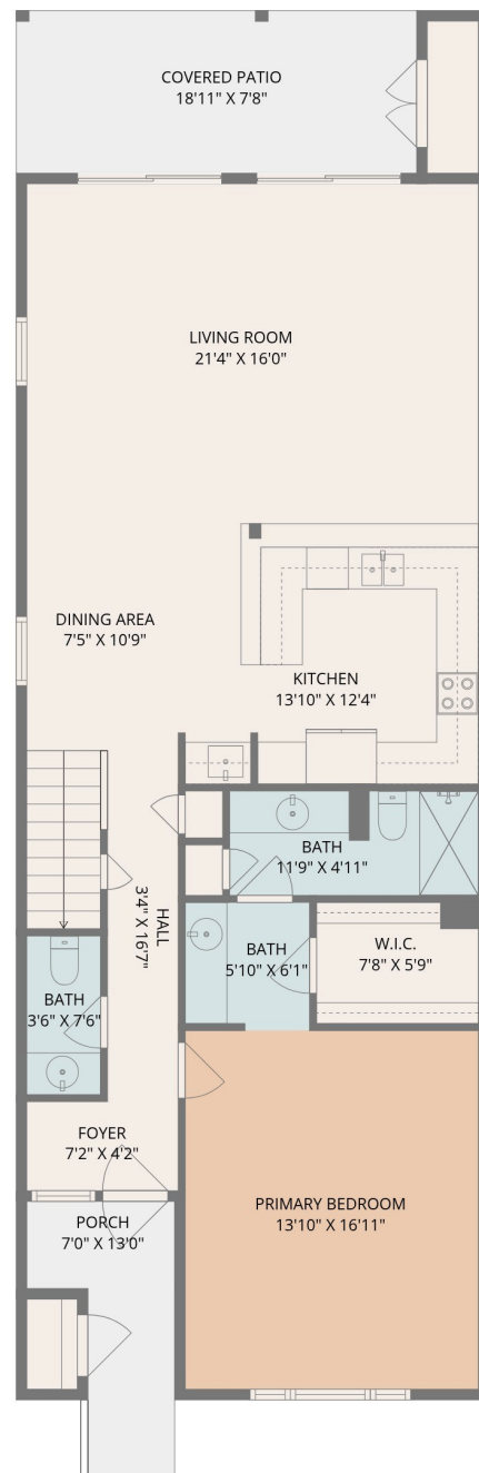
1ST FLOOR
