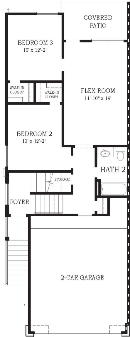
FIRST FLOOR
