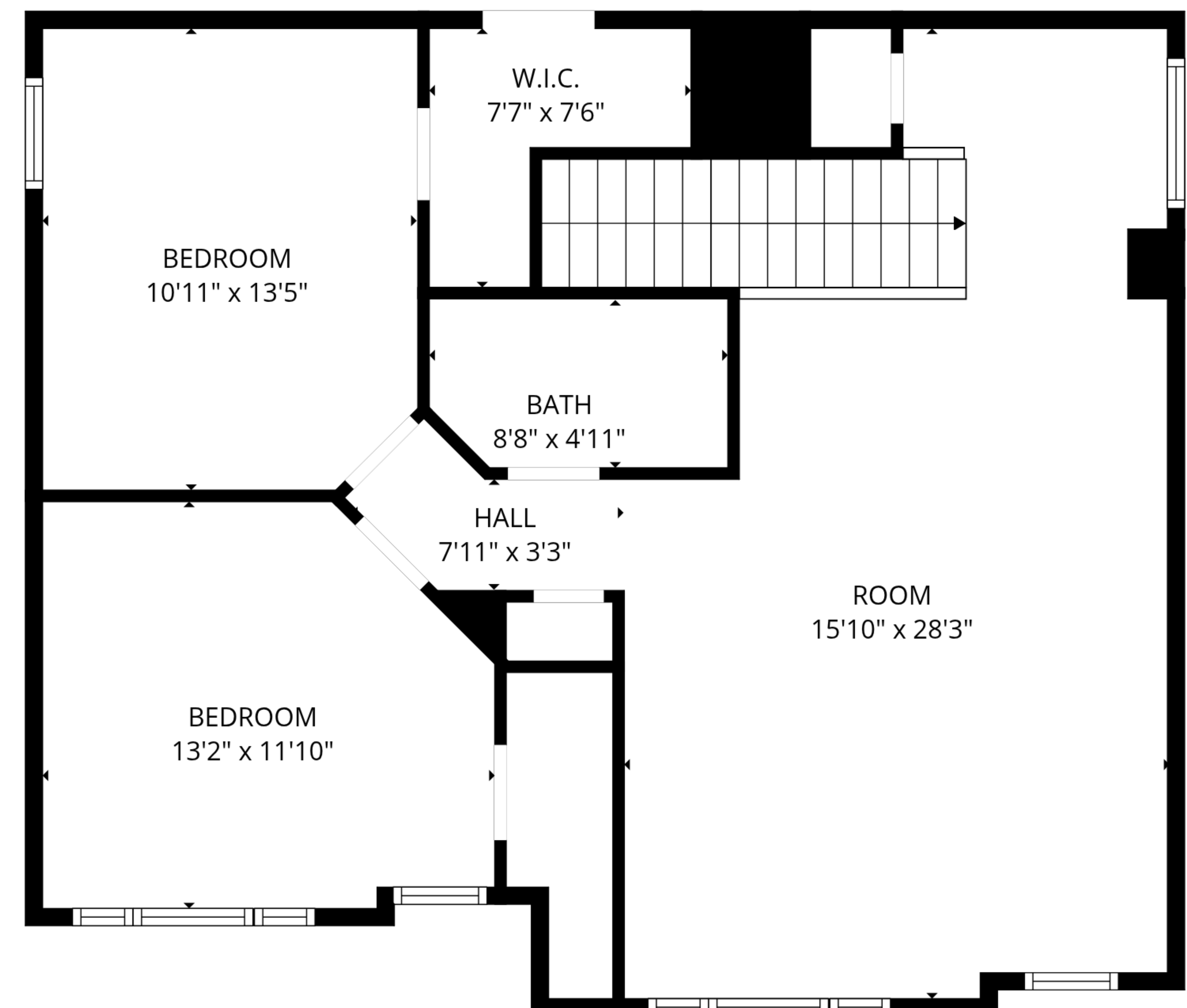
2nd floor
